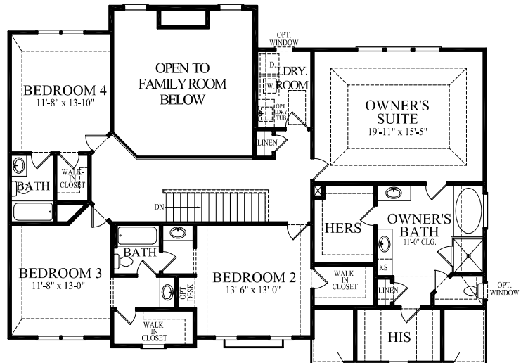
SECOND FLOOR
