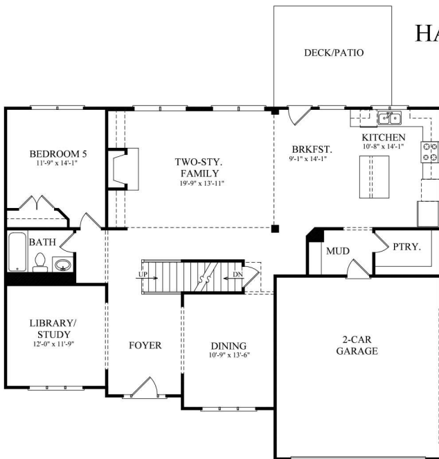
HAMPTON FIRST FLOOR
